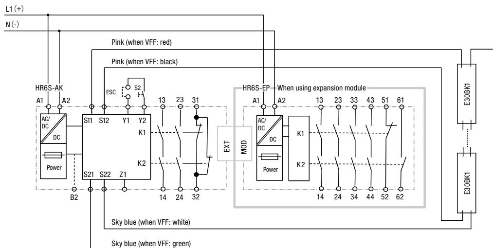
Up to 24 series connection
